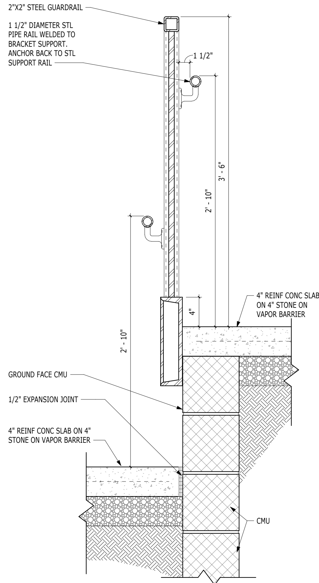
6 DETAIL 1 1/2" = 1'-0"
