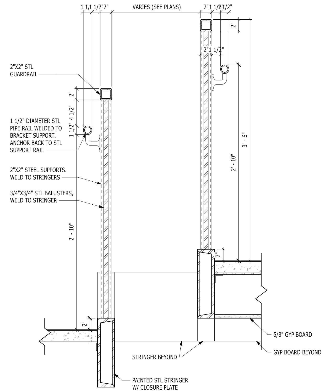
4 DETAIL 1 1/2" = 1'-0"
