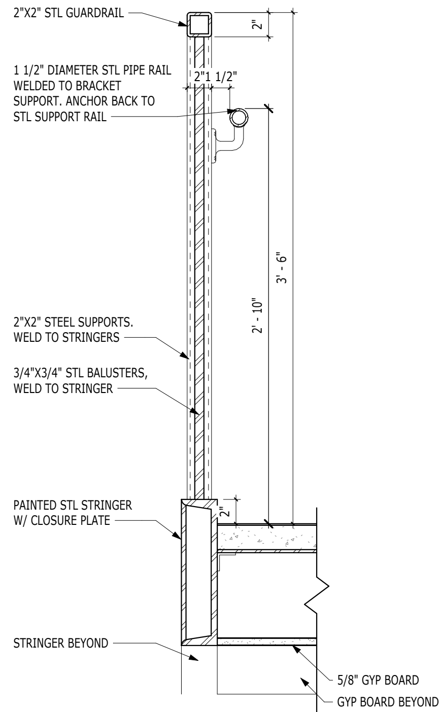
3 DETAIL 1 1/2" = 1'-0"
