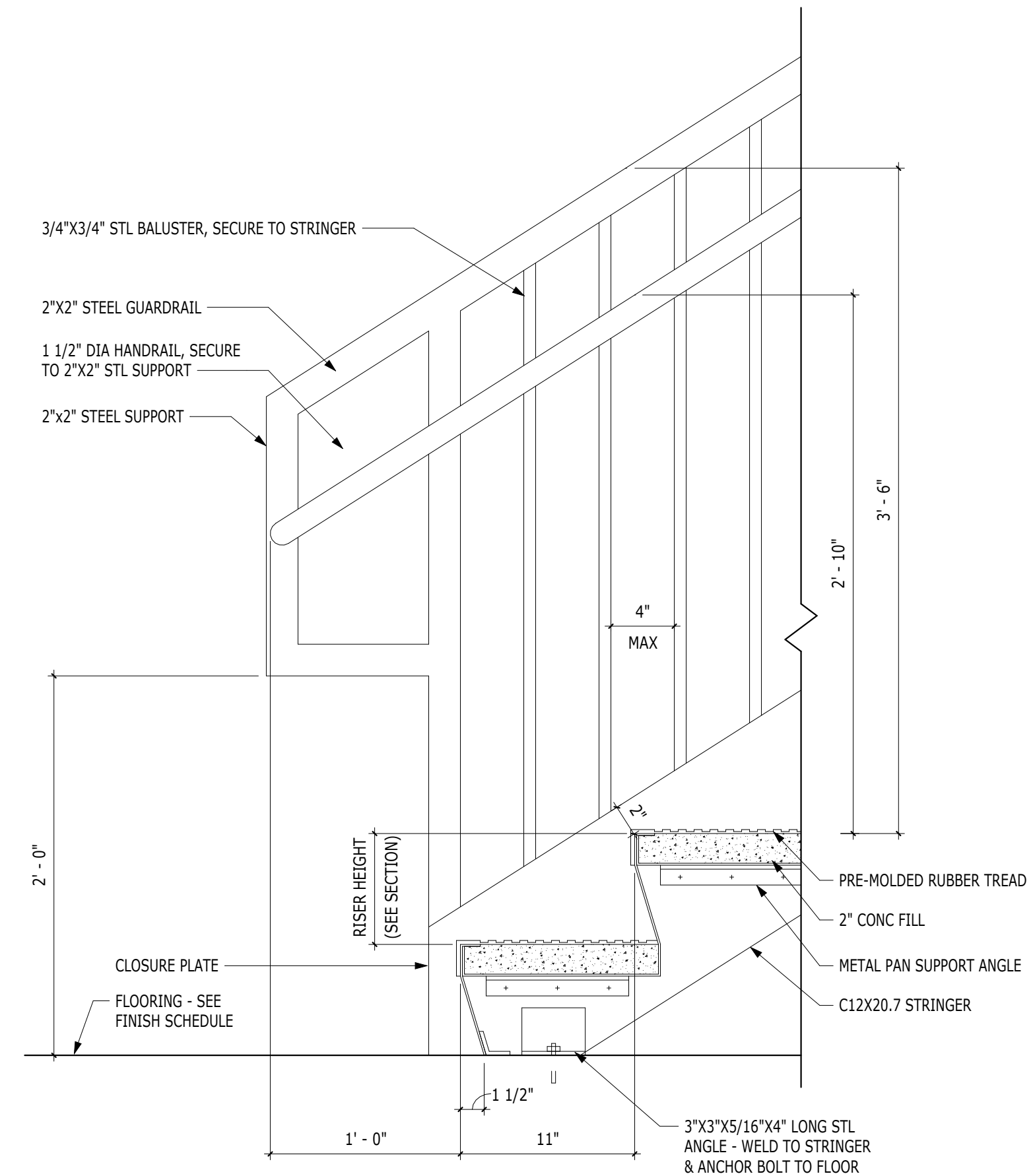
7 DETAIL 1 1/2" = 1'-0"
