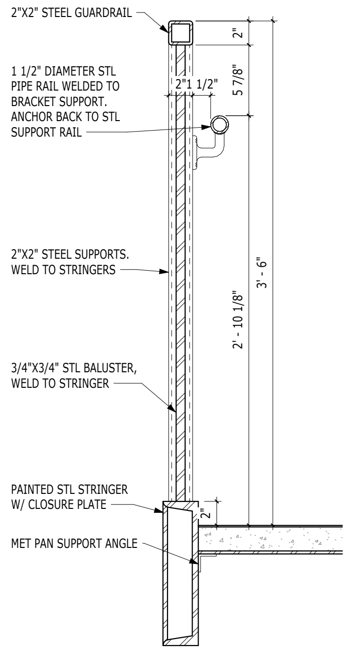
1 DETAIL 1 1/2" = 1'-0"
