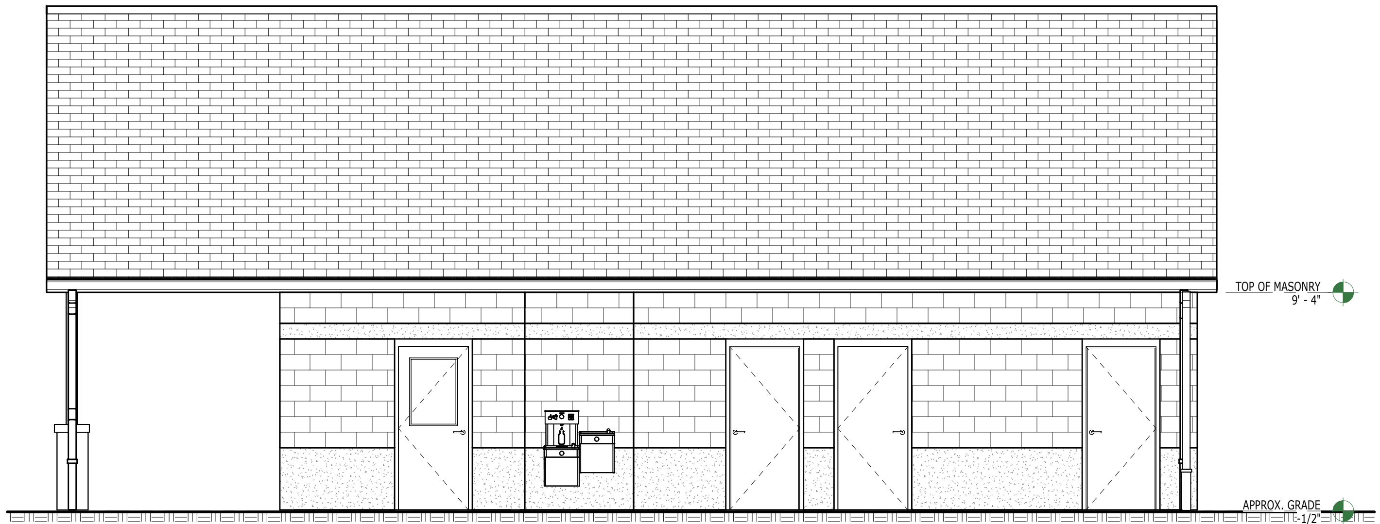
4 ELEVATION 1/4" = 1'-0"
