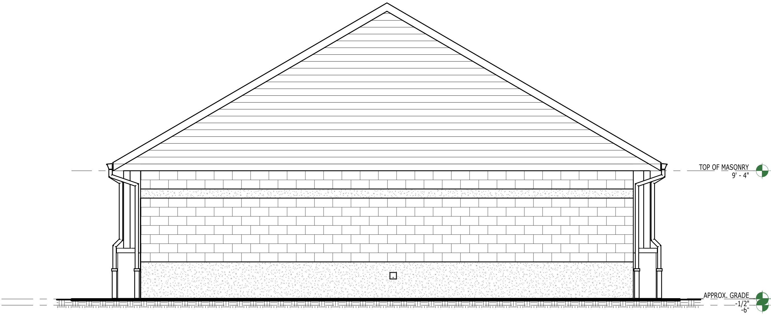
1 ELEVATION 1/4" = 1'-0"
