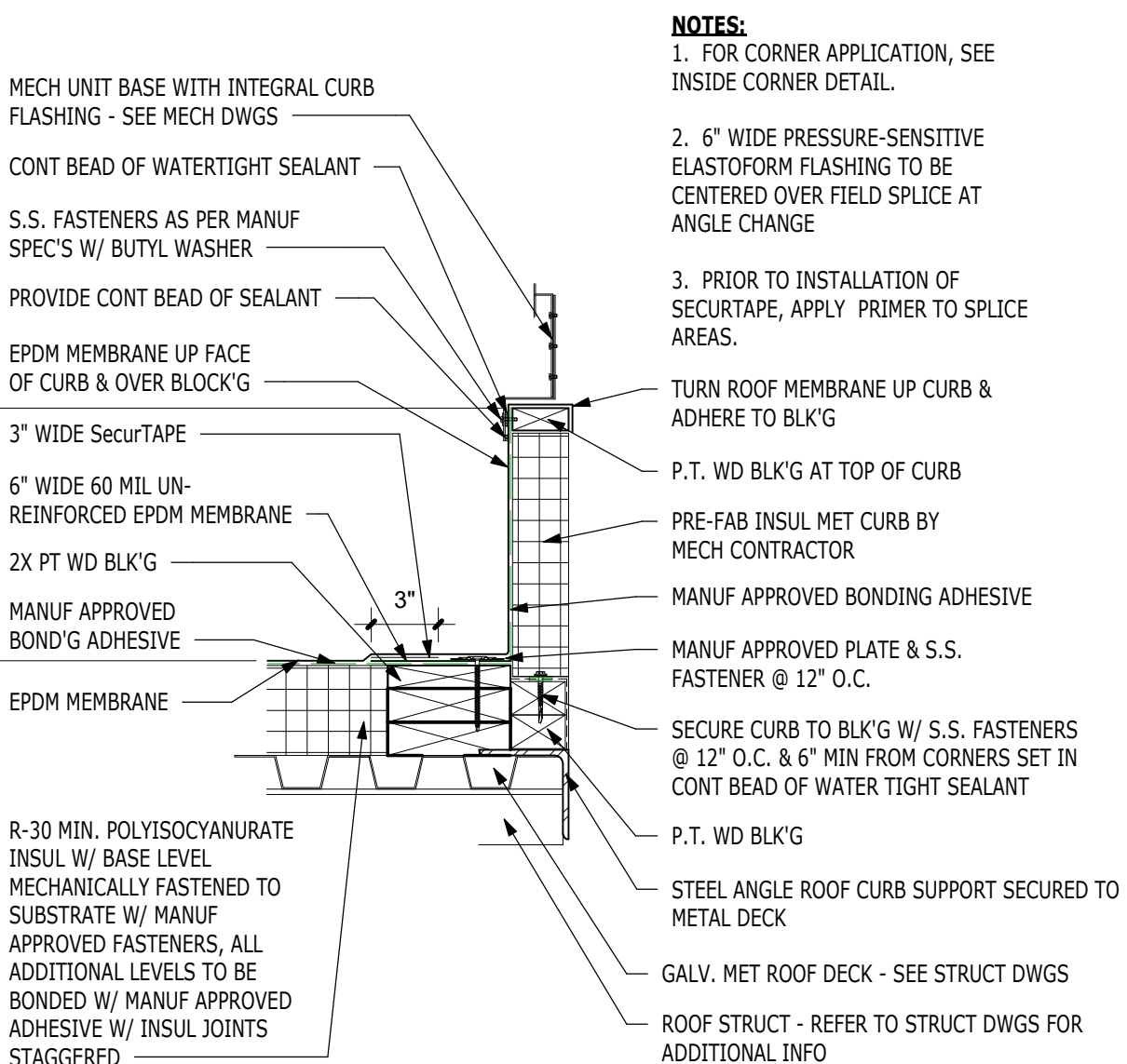
6 EPDM ROOF CURB DETAIL 1 1/2" = 1'-0"
