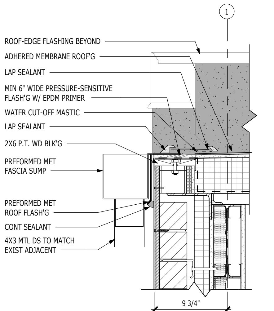
11 SCUPPER DETAIL 1 1/2" = 1'-0"
