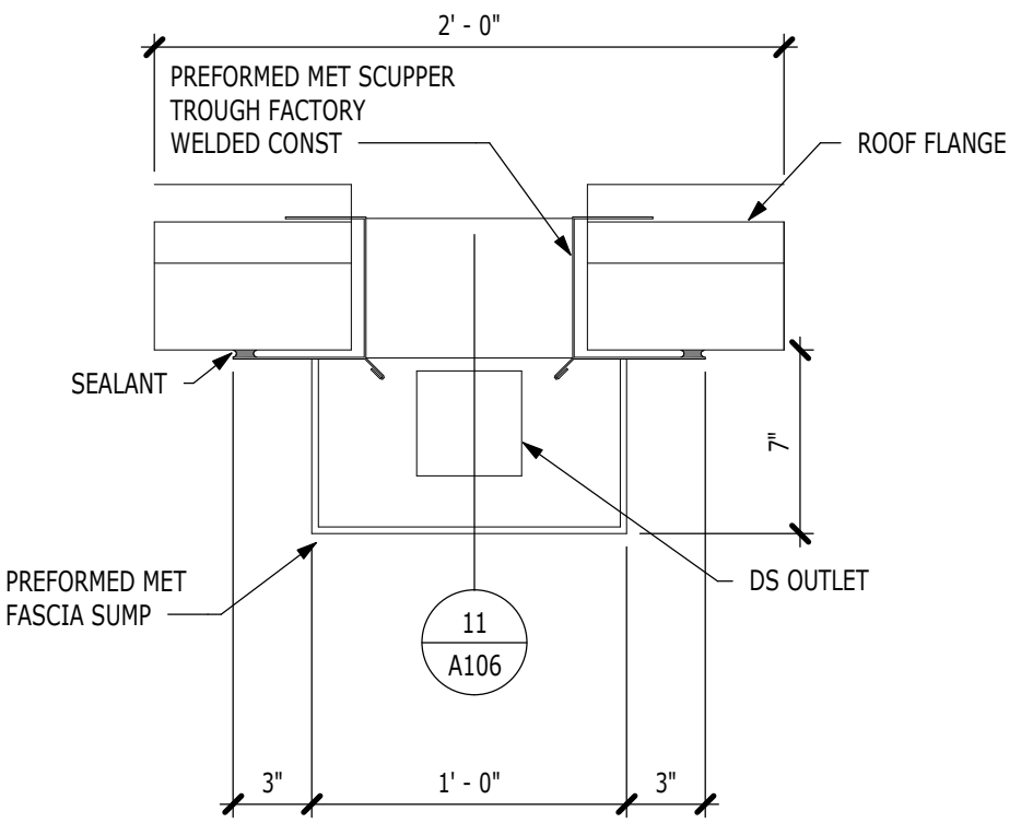
9 SCUPPER PLAN 1 1/2" = 1'-0"
