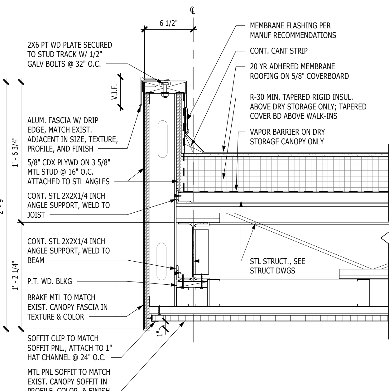
13 TYP. FASCIA DETAIL 1 1/2" = 1'-0"
