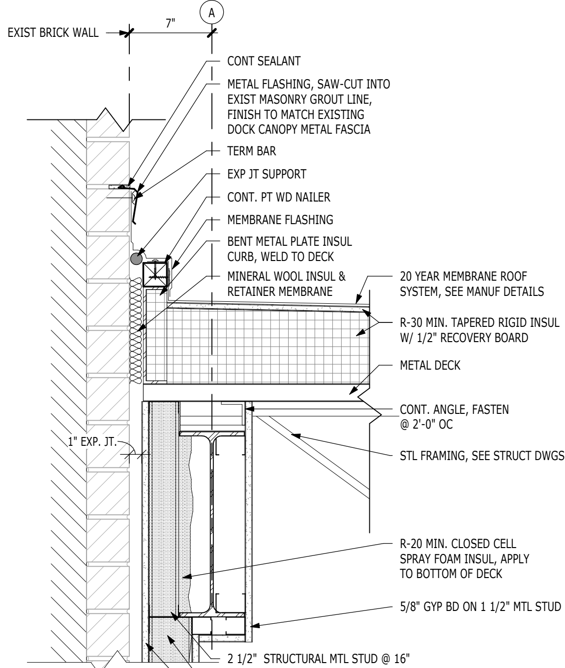
2 DETAIL 1 1/2" = 1'-0"
