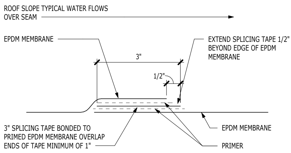
7 EPDM LAP SEAM DETAIL 6" = 1'-0"
