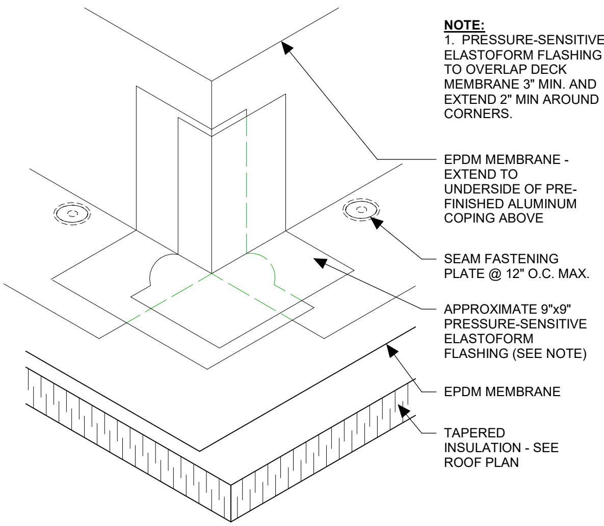
3 EPDM OUTSIDE CORNER DETAIL 1 1/2" = 1'-0"
