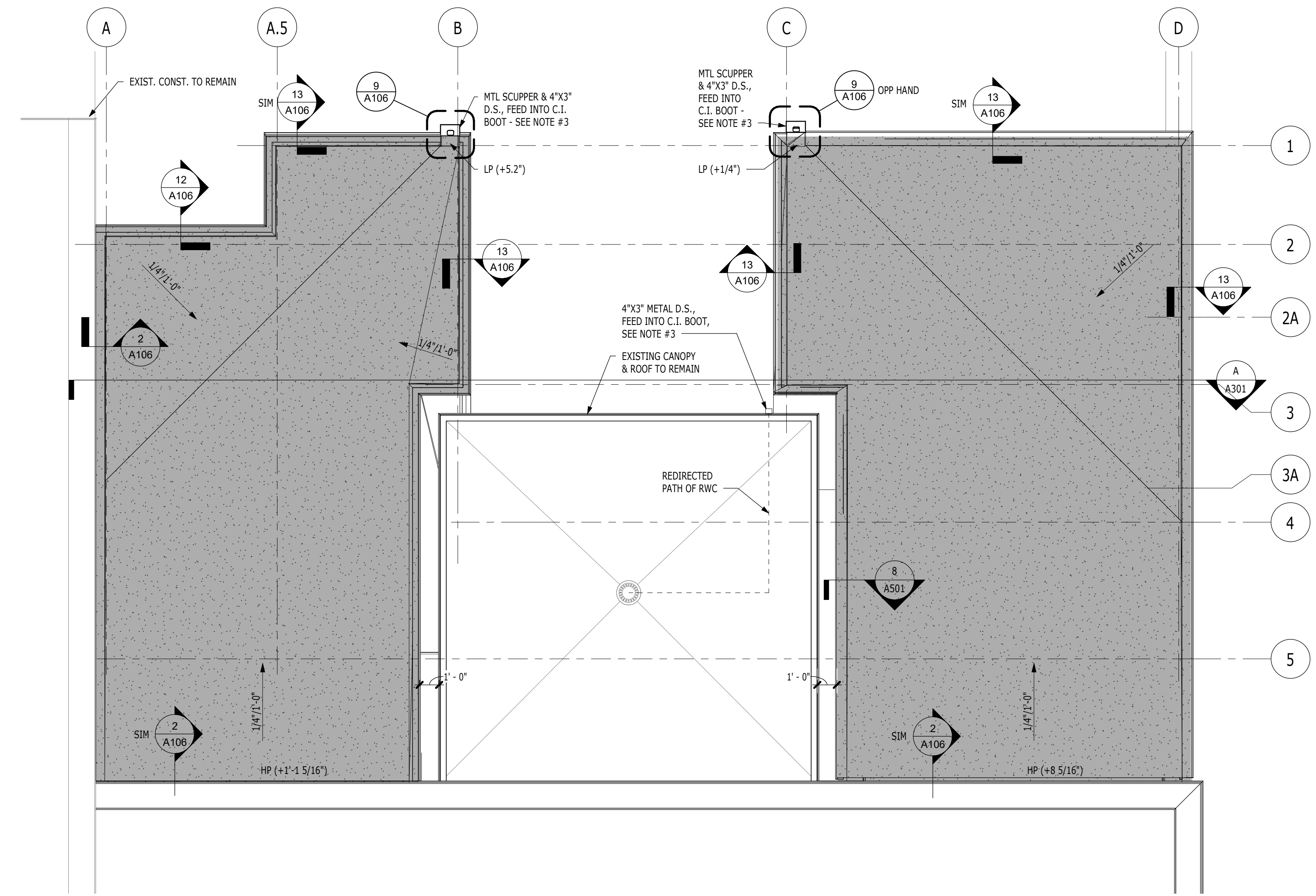
1 ROOF PLAN 1/4" = 1'-0"
