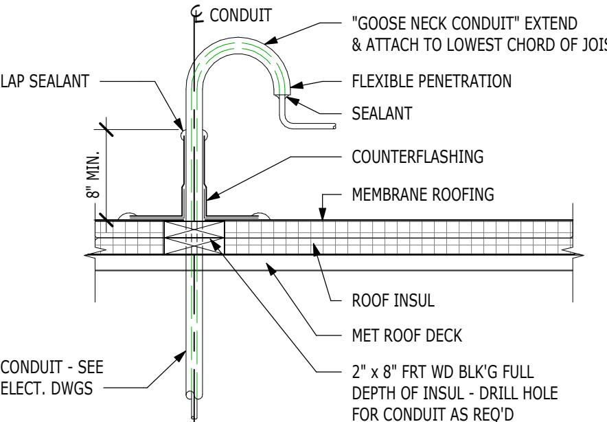
8 CONDUIT PENETRATION DETAIL 1" = 1'-0"
