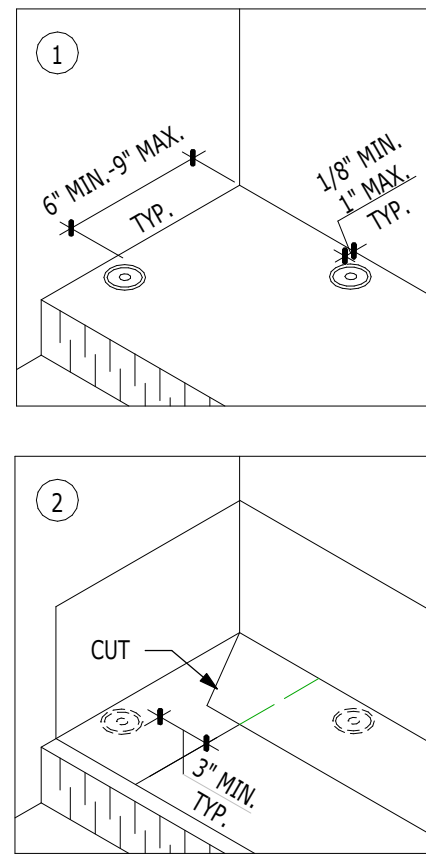
4 EPDM INSIDE CORNER DETAIL 1 1/2" = 1'-0"
