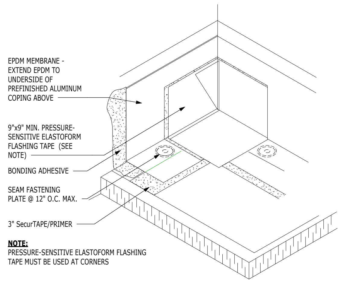
4 EPDM INSIDE CORNER DETAIL 1 1/2" = 1'-0"
