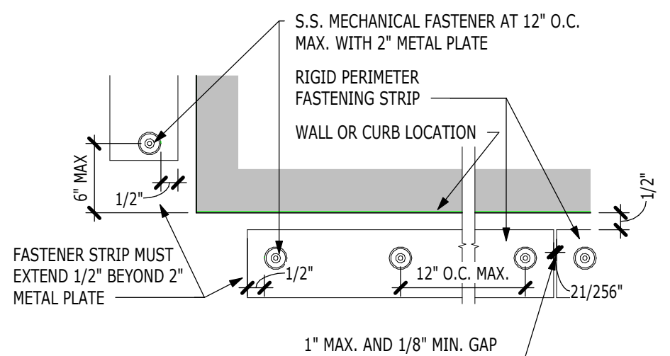
OUTSIDE CORNER PLACEMENT
