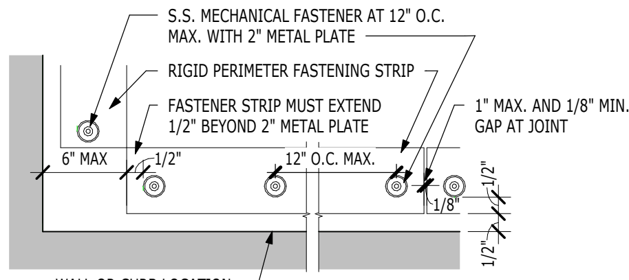
INSIDE CORNER PLACEMENT
