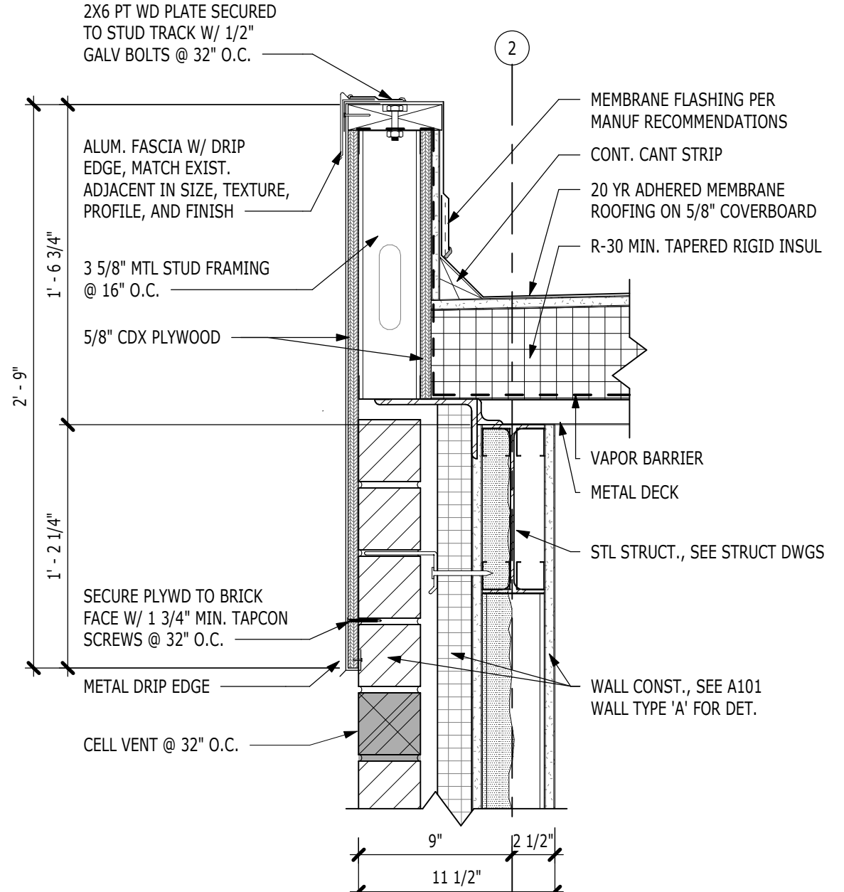
12 FASCIA DETAIL 1 1/2" = 1'-0"
