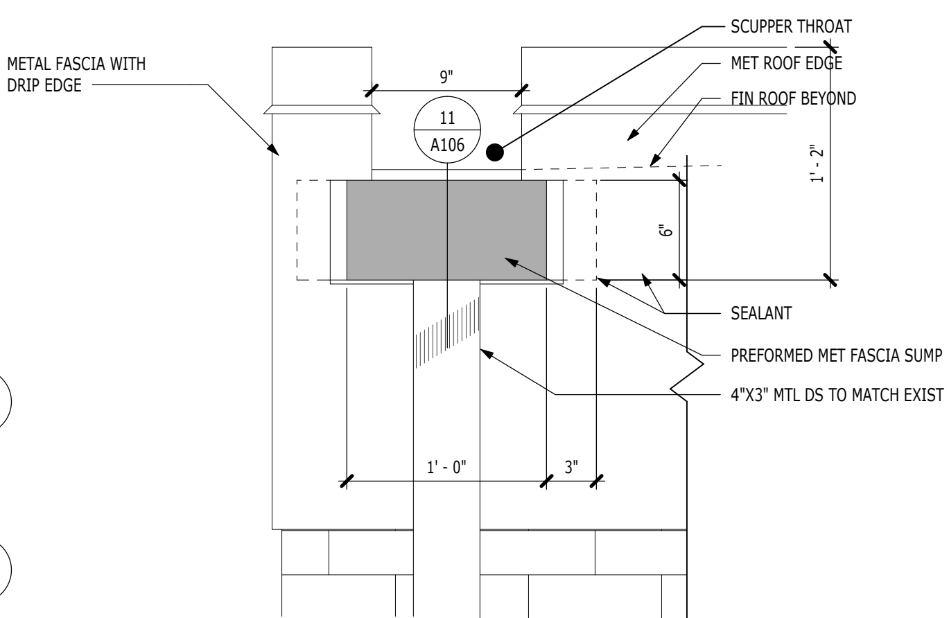
10 SCUPPER ELEVATION 1 1/2" = 1'-0"
